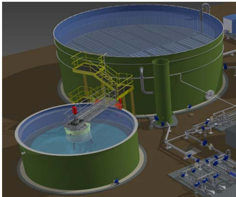
ACWA settlement tank and aeration tank during design
